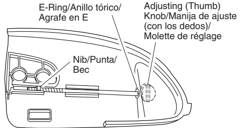
Figure 6 - Turning Adjusting Knob on Model 107625-01, -02
